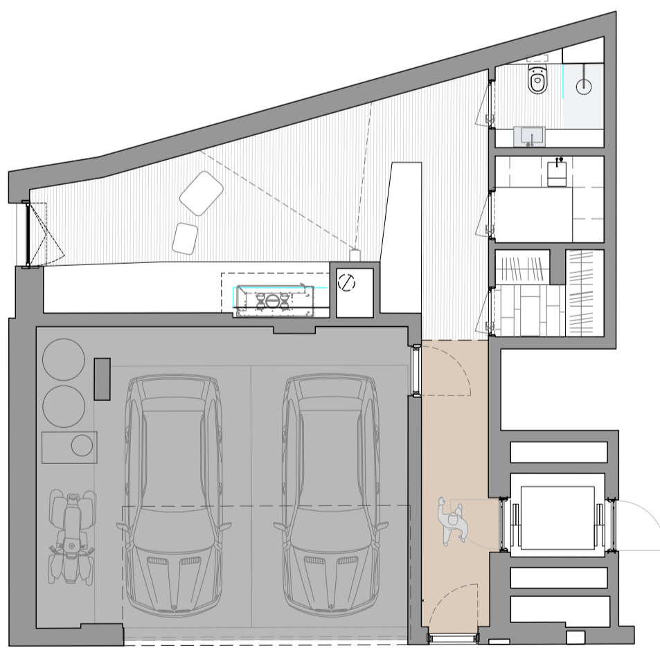
Planta entrada / Entrance floor
